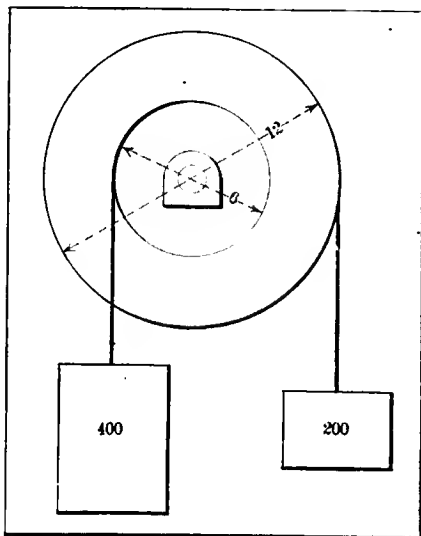
Fig. 2—Balanced weights on shaft and two drums
